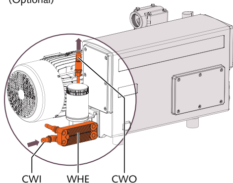
Air-cooled motor version (Optional)
