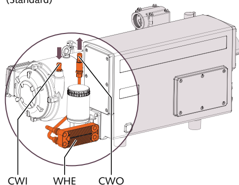
Water-cooled motor version (Standard)
